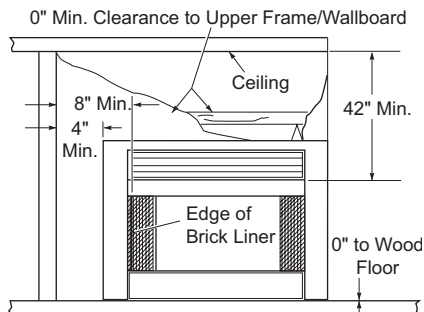
Figure 5 - Minimum Clearance Front View
