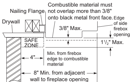
Figure 9 - Framing for Built-In Firebox Installation, Top View
