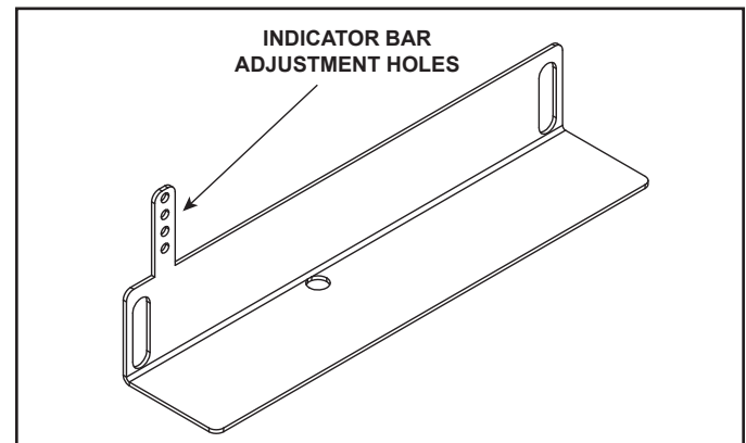
Figure 4.12 Baffle Adjustment - PVI-SLP
