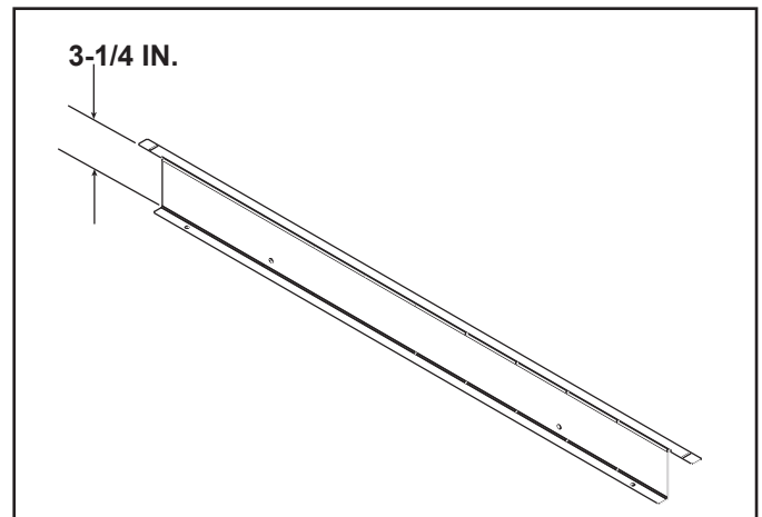
Figure 10.3 Top Finishing Template Bend - LMOD Series Doors
