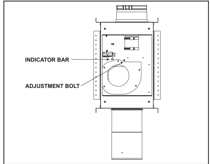
Figure 4.11 Baffle Adjustment Location - PVI-SLP
