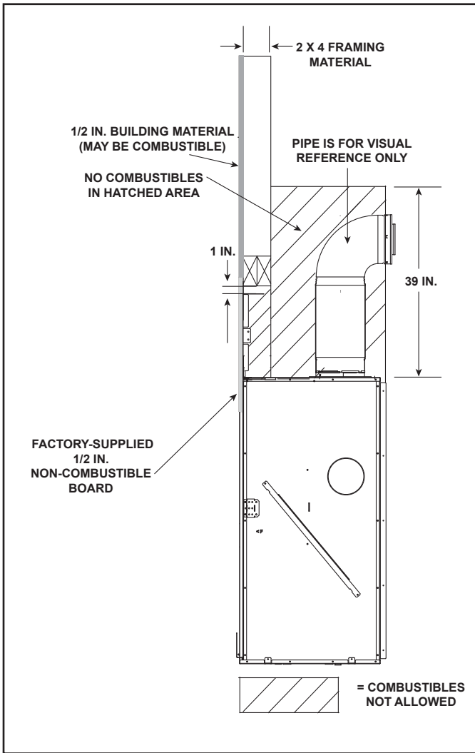
→ Figure 10.11 Non-Combustible Zone
